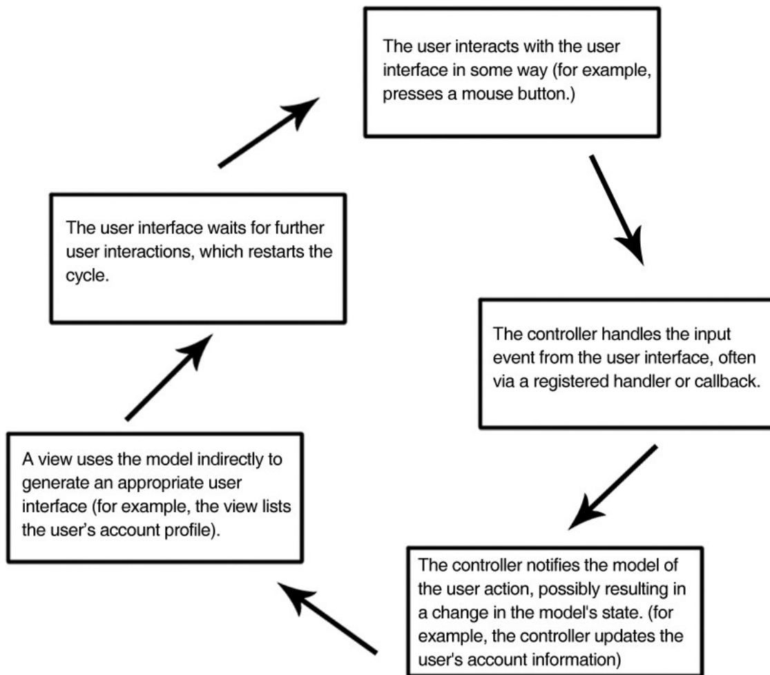
Fig. 14 CakePHP Flowchart
