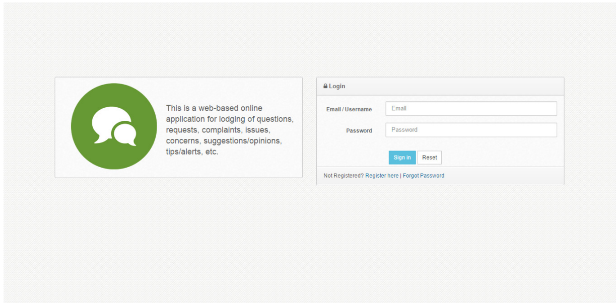
Figure 8: Login page
