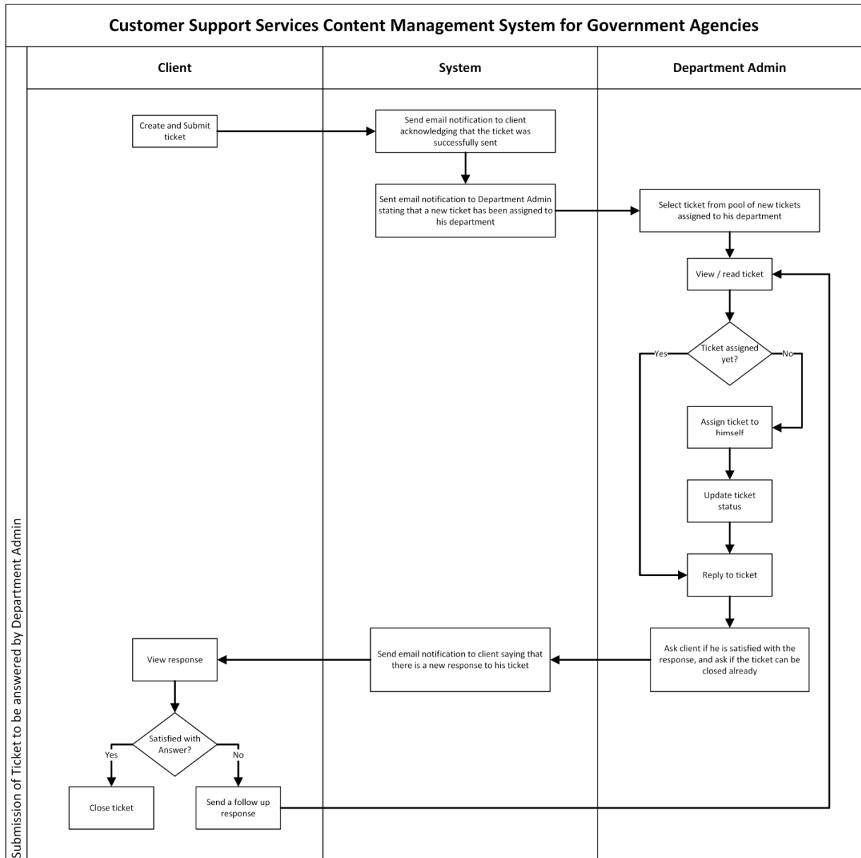
Figure 4: Submission of Ticket to be answered by Department Admin
