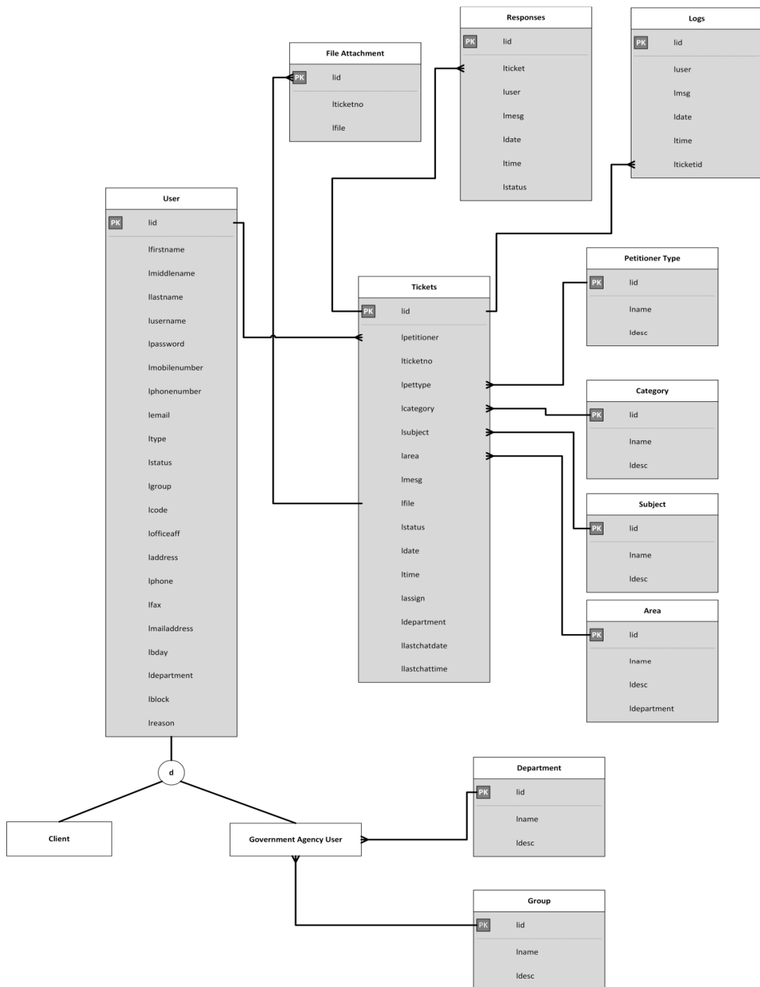
Figure 7: Entity Relationship Diagram
