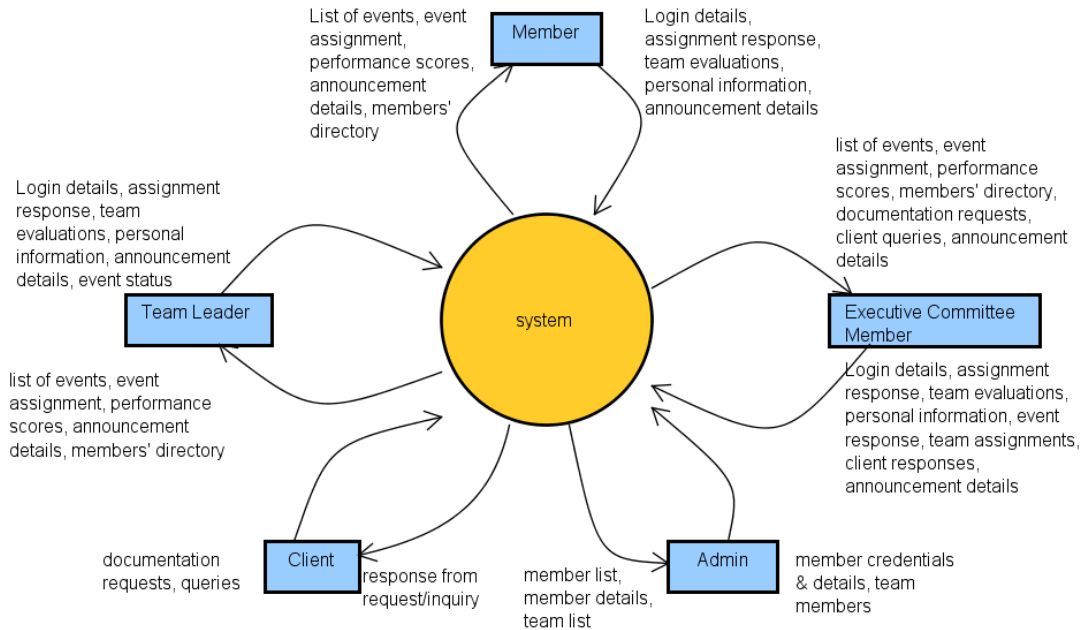
Figure 3: Context Diagram
