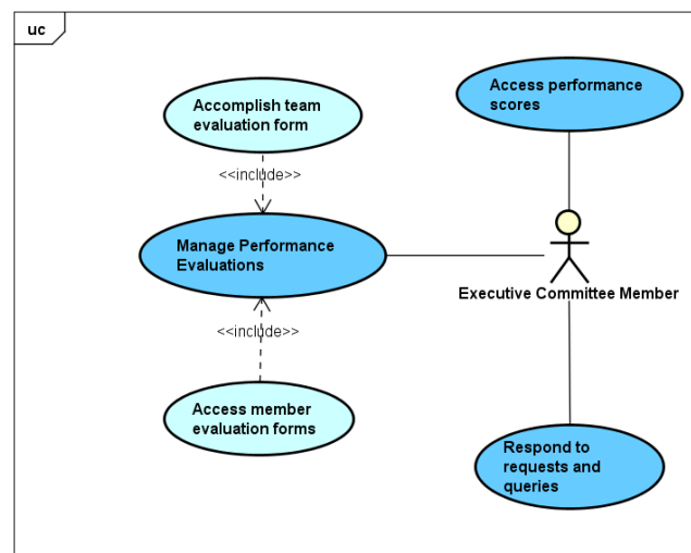
Figure 6: Use Case Diagram, Executive Committee member functionalities
