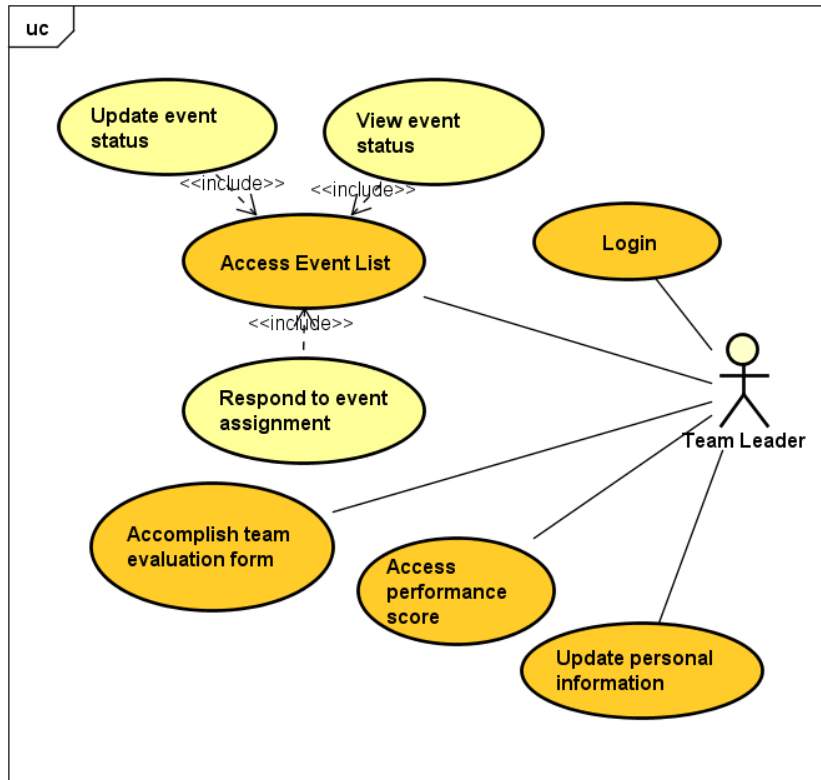
Figure 5: Use Case Diagram, Team Leader functionalities
