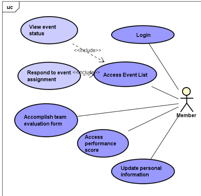
Figure 4: Use Case Diagram, Member functionalities
