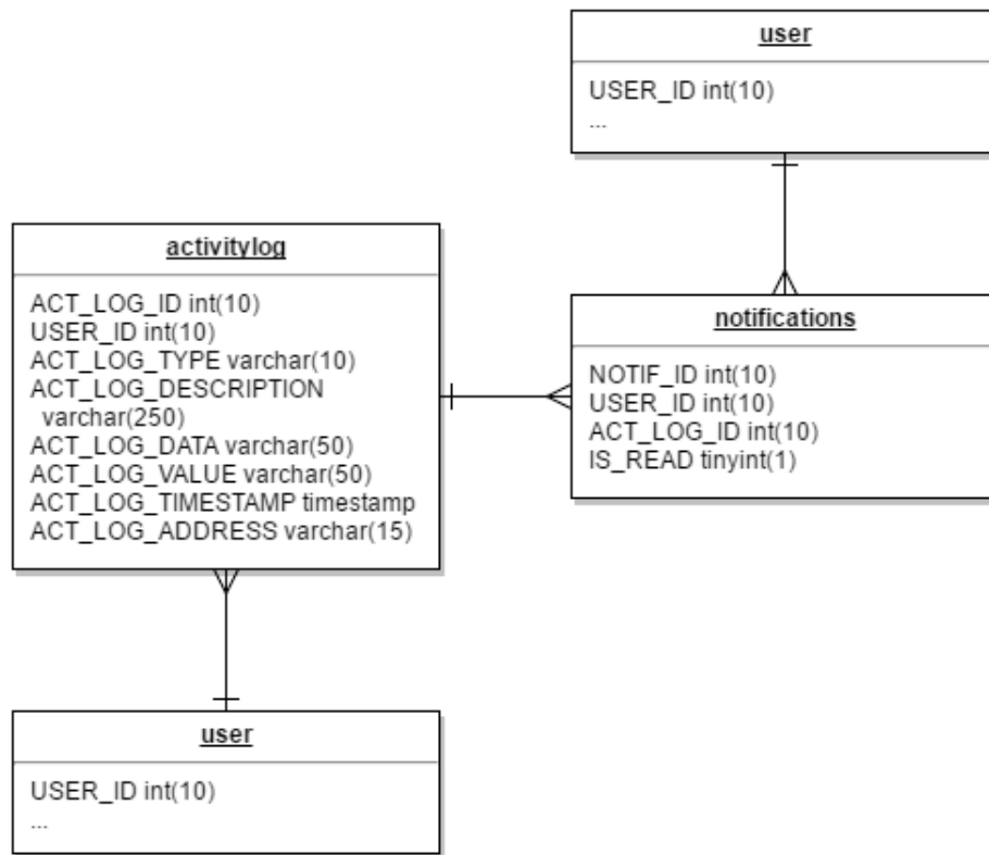
Figure 11: Entity Relationship Diagram (ERD) (Activity)
