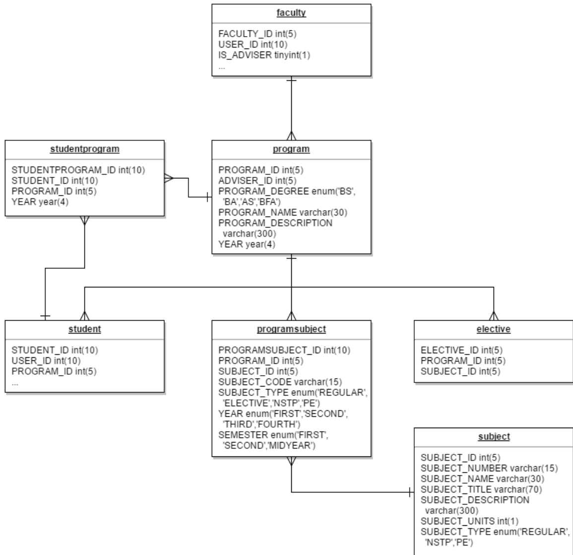
Figure 8: Entity Relationship Diagram (ERD) (Program)
