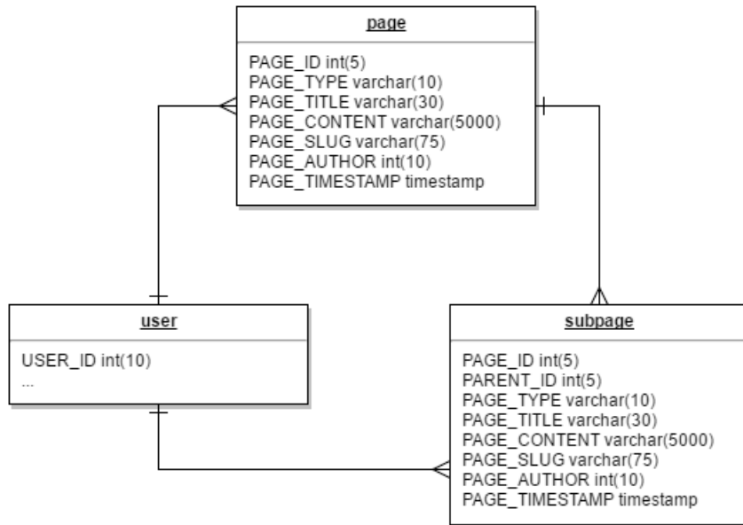
Figure 9: Entity Relationship Diagram (ERD) (Page)
