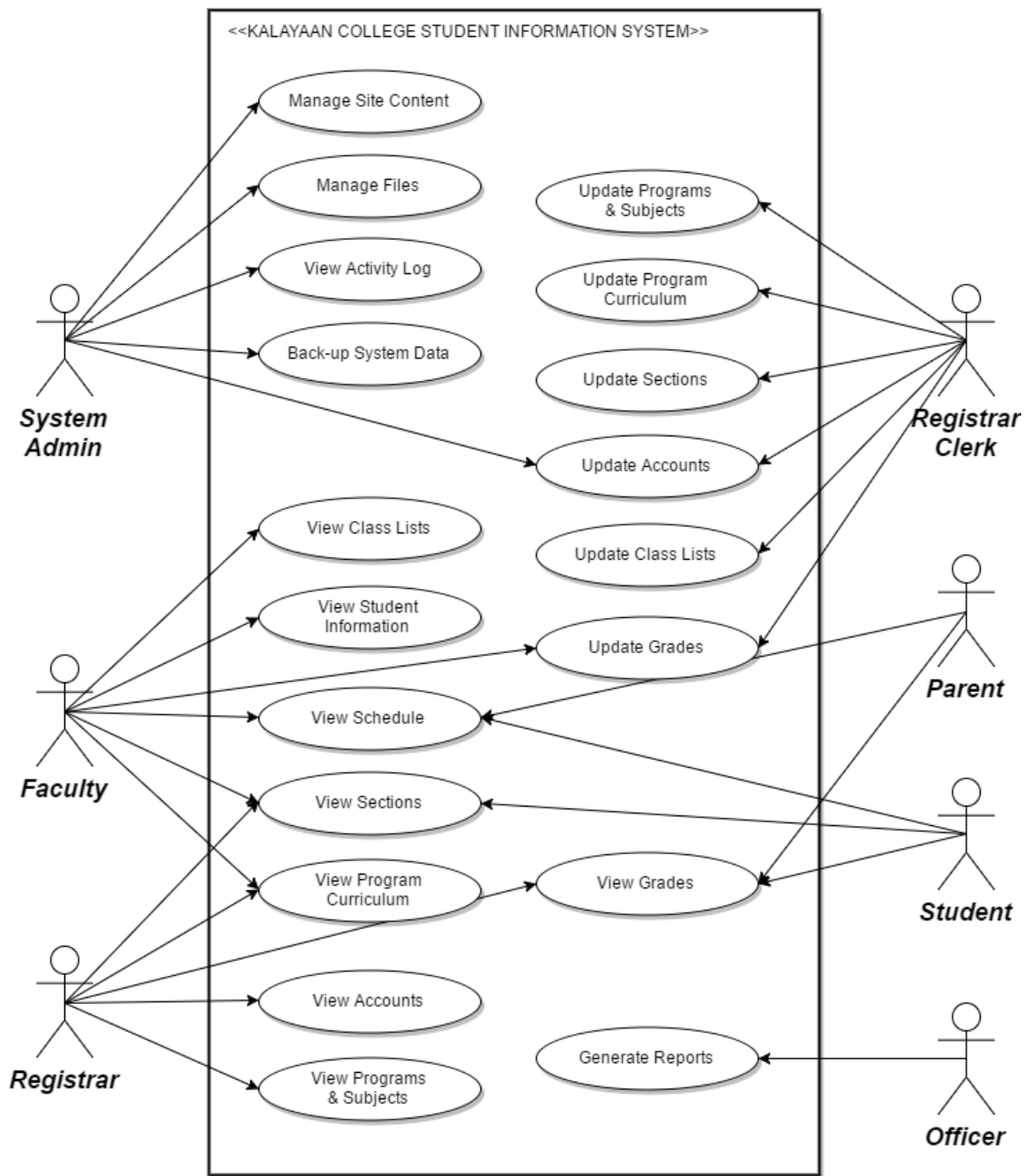
Figure 4: Use Case Diagram for KSIS
