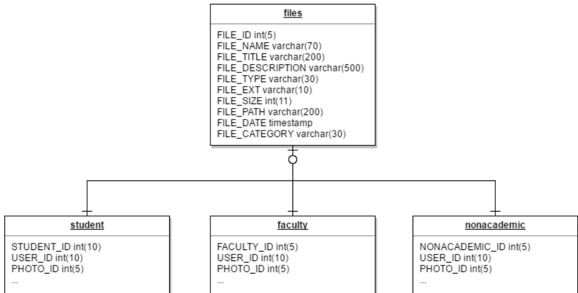
Figure 10: Entity Relationship Diagram (ERD) (Files)
