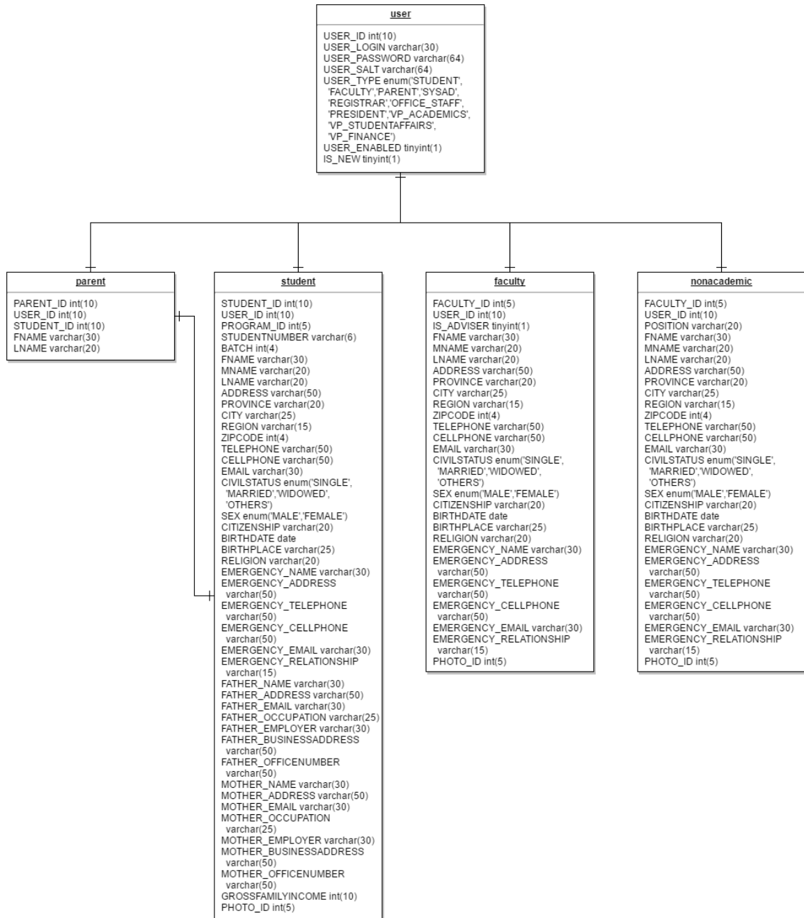
Figure 6: Entity Relationship Diagram (ERD) (User)
