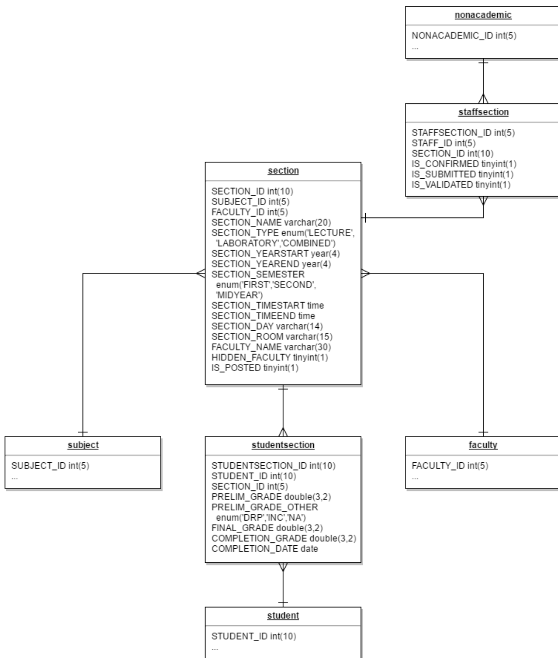
Figure 7: Entity Relationship Diagram (ERD) (Section)
