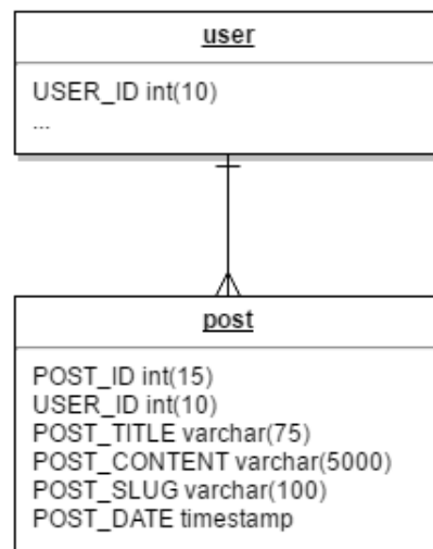
Figure 12: Entity Relationship Diagram (ERD) (Post)
