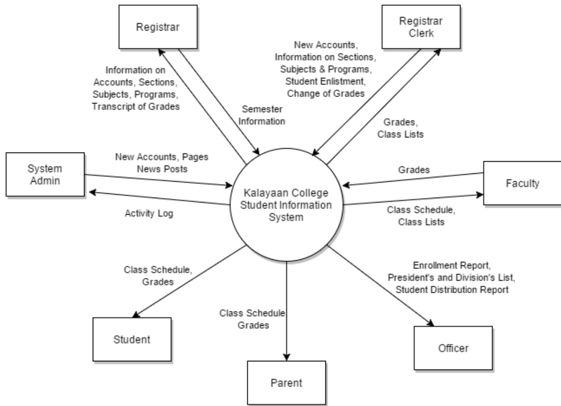
Figure 1: Context Diagram for KSIS
