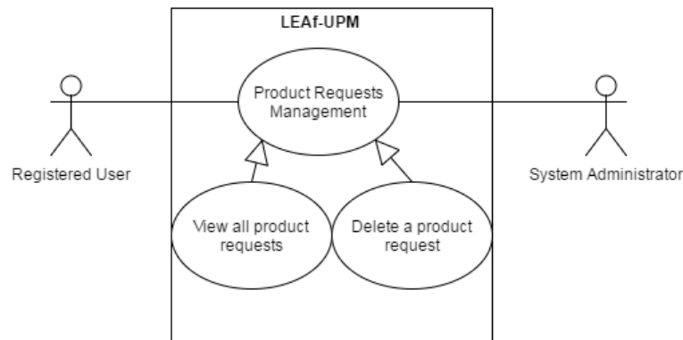
Figure 14: Product Requests Management Use Case Diagram
