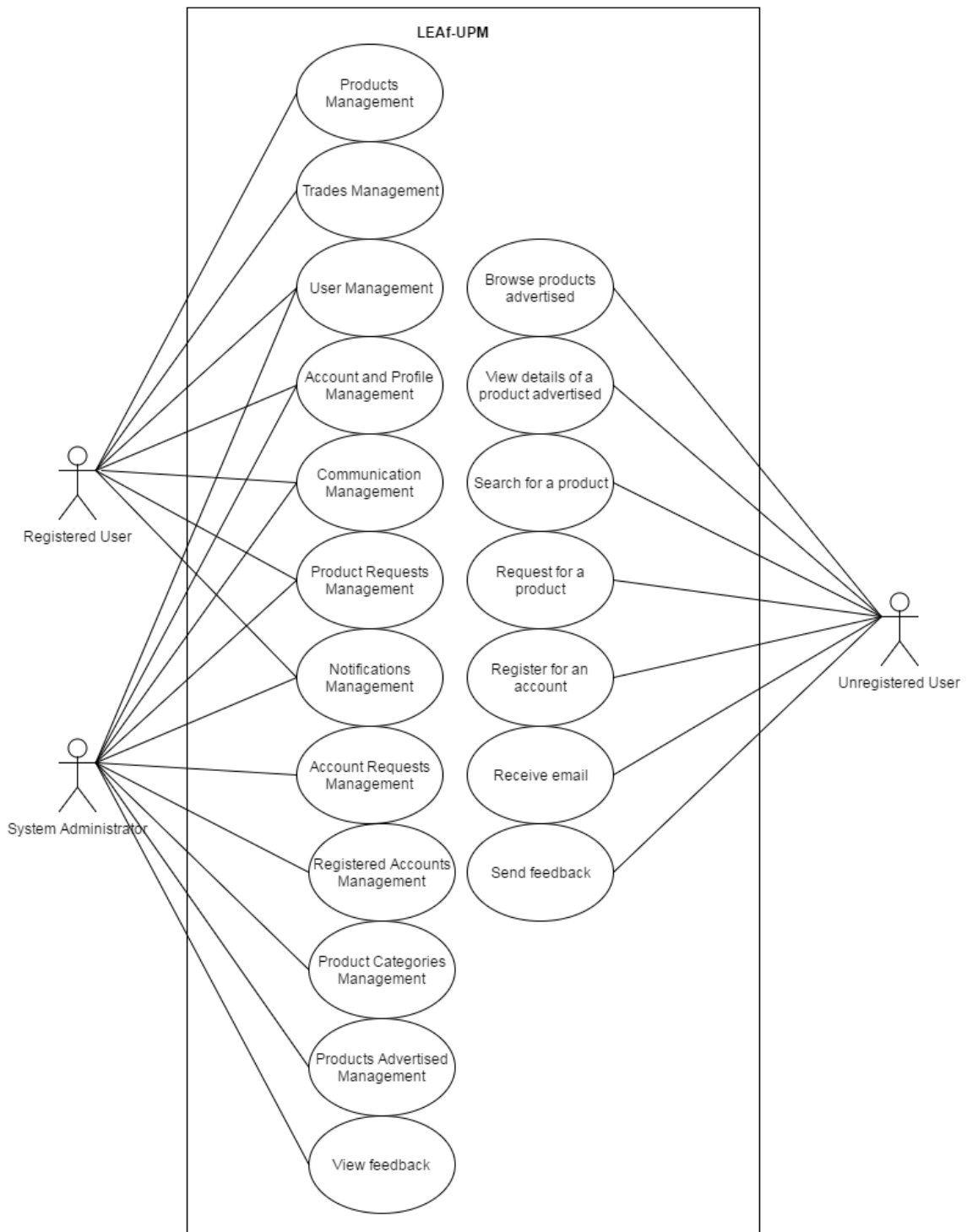
Figure 5: Top-level Use Case Diagram
