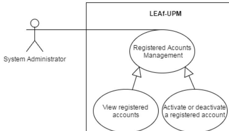
Figure 11: Registered Accounts Management Use Case Diagram
