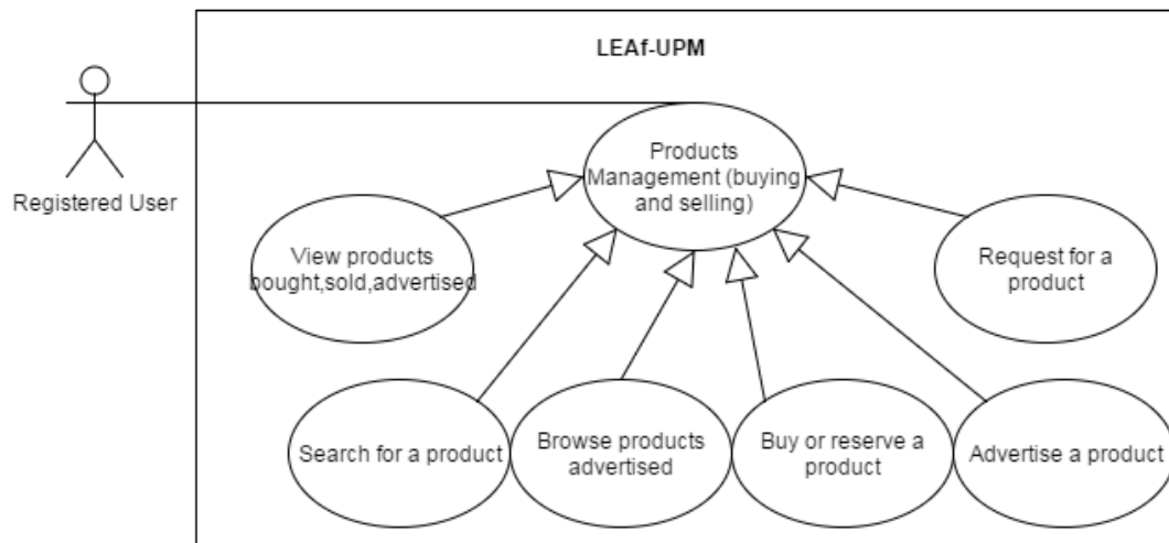
Figure 6: Products Management Use Case Diagram
