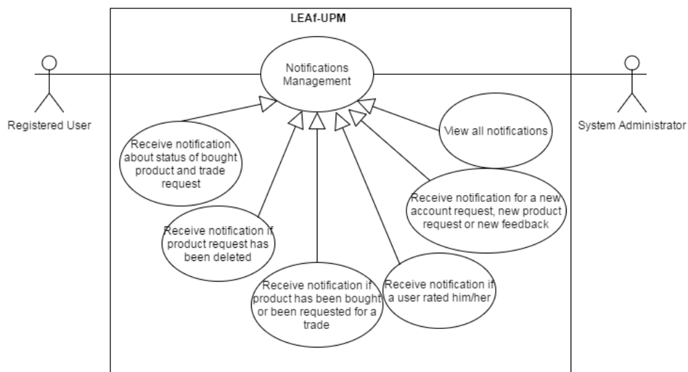
Figure 15: Notifications Management Use Case Diagram
