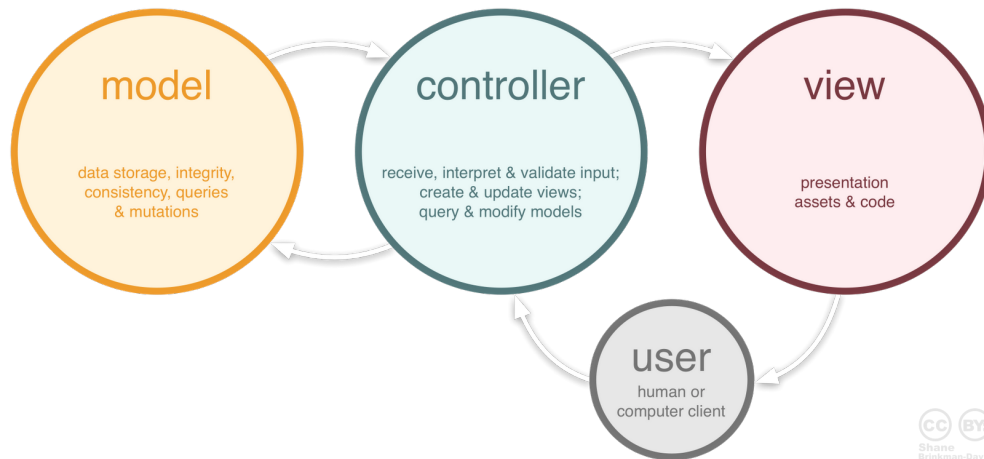
Figure 3: Model-View-Controller
