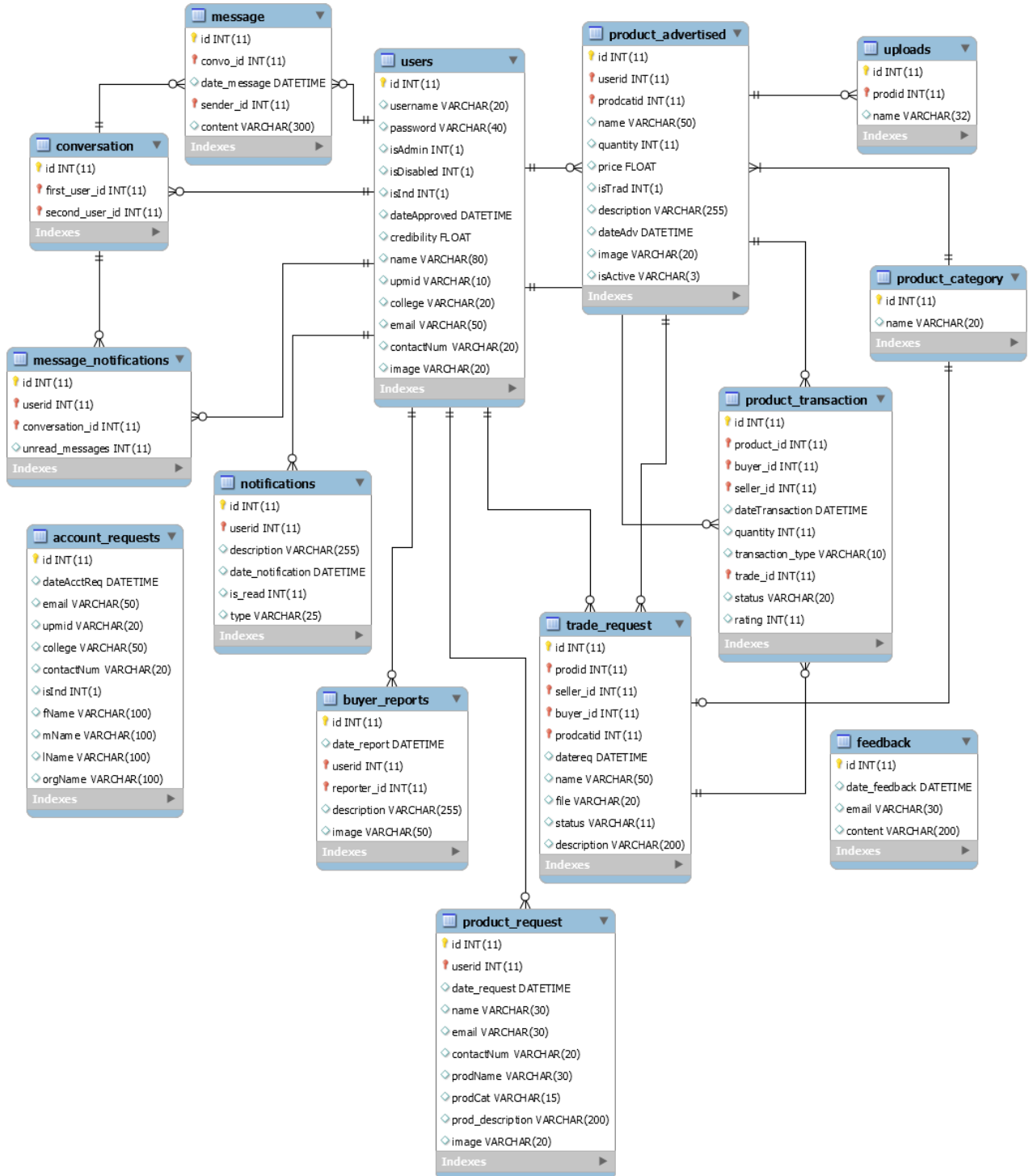
Figure 16: Entity Relationship Diagram
