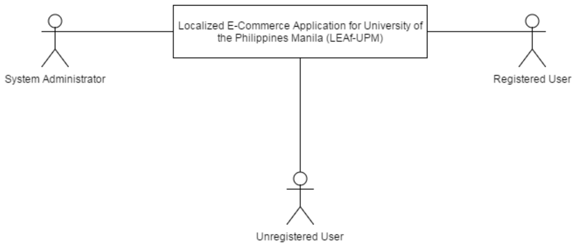
Figure 4: Context Diagram
