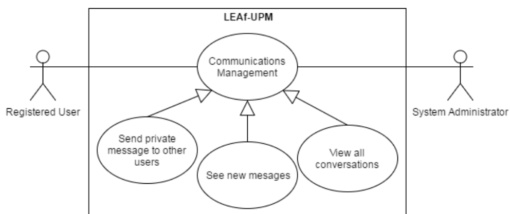
Figure 13: Communications Management Use Case Diagram
